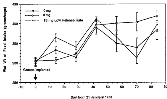
FIG. 1 Mean wet weight of feed consumption ( \pm SEM) measured at 14 day intervals from 21 January to 14 April in three groups implanted with 0, 8 and 18 mg of melatonin.
